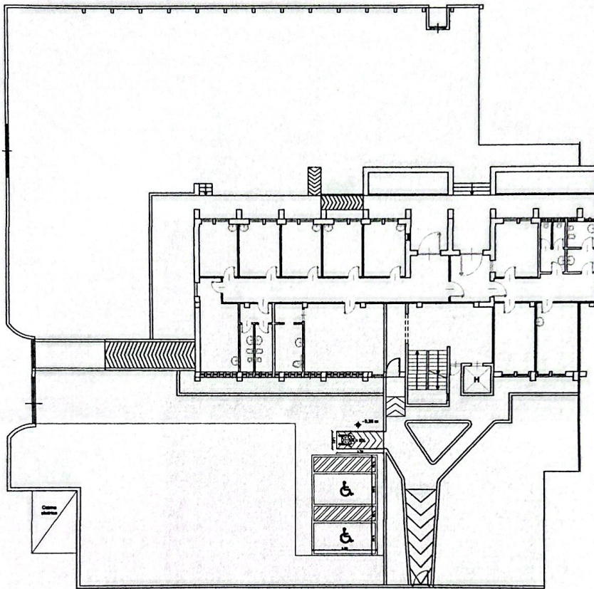
PIANO TERRA Scale 1:100
